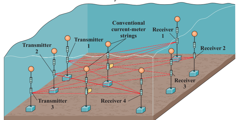
FIGURE 3-17 A typical acoustic tomography array. Sound pulses sent from each transmitter are received by each of the receivers.
