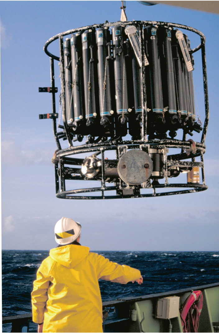
FIGURE 3-12 Rosette water sampler. The sample bottles, some fitted with thermometer racks, are arranged in a rosette pattern around an electronic device that enables researchers on the ship above to close individual sample bottles at selected depths through an electrical signal sent down the hydrographic cable. The round frame below the water-sampling bottle rack usually contains a CTD and possibly other sensors, such as turbidity-measuring devices.
