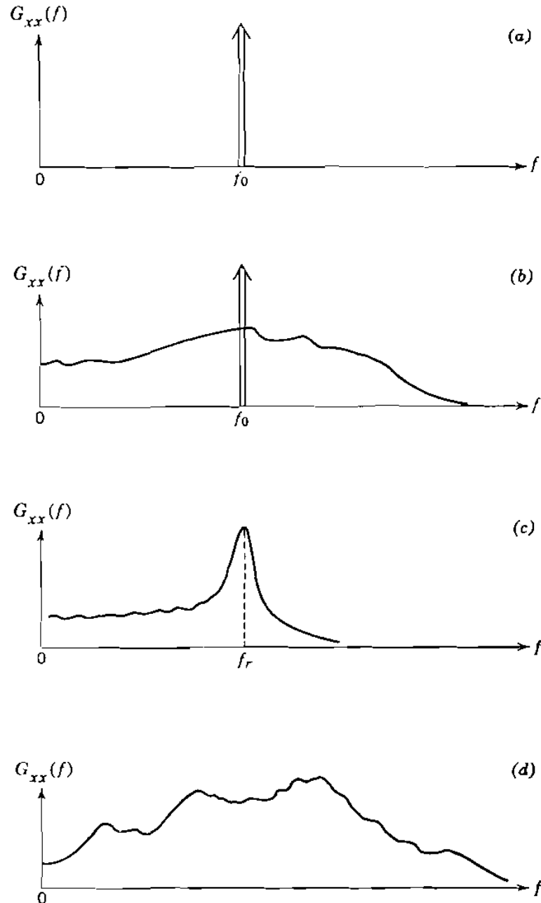
Figure 1.14 Autospectral density function plots. (a) Sine wave. (b) Sine wave plus random noise. (c) Narrow-band random noise. (d) Wide-band random noise.
