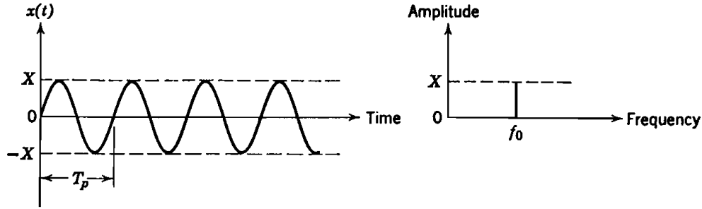
Figure 1.3 Time history and spectrum of sinusoidal data.
