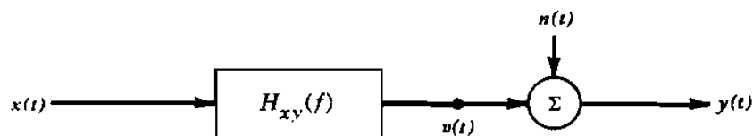
Figure 1.15 Single-input/single-output system with output noise.
