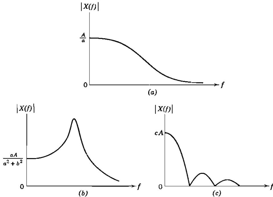
Figure 1.7 Spectra of transient data.
