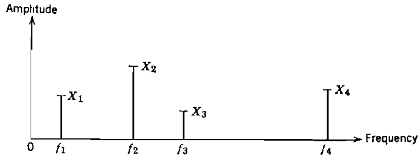
Figure 1.5 Spectrum of almost-periodic data.
