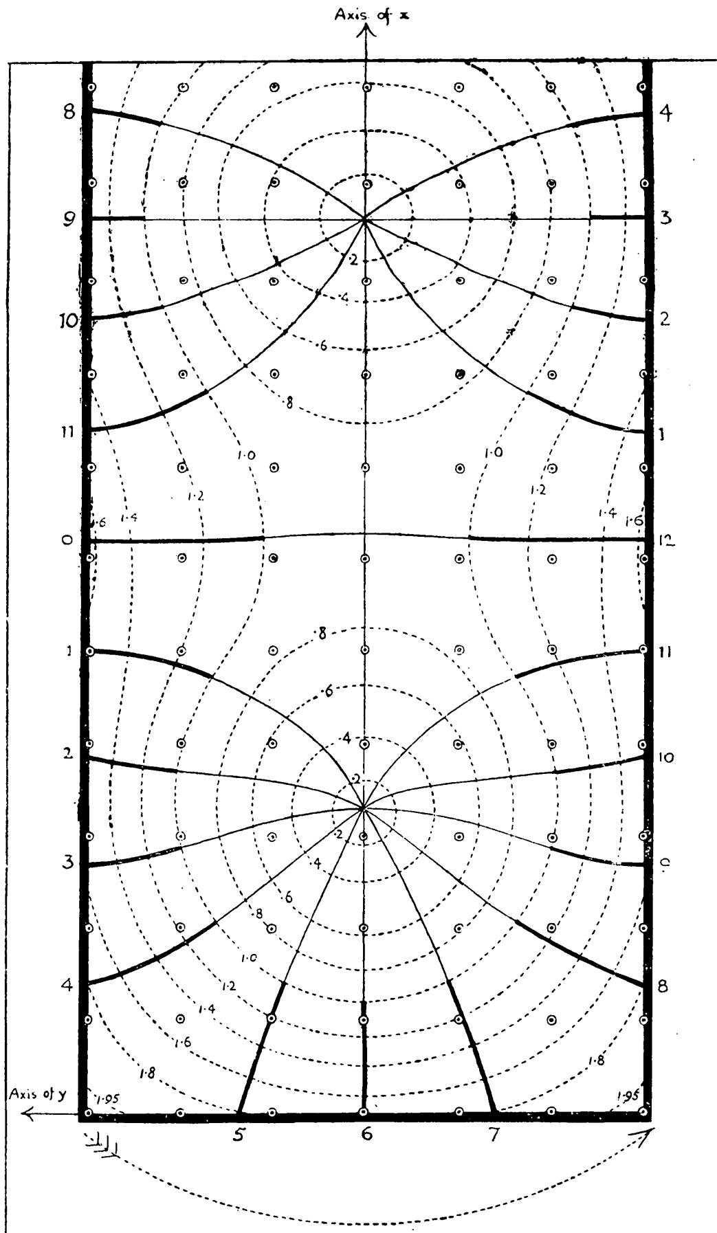
FIG. 1.—Cotidal lines in basin where a Kelvin wave is being reflected.—Full lines are cotidal lines. Figures outside the edge of the basin show time of high water on corresponding cotidal line. Dotted lines are lines of equal tidal range. Figures inside basin show amount of tidal range. Small circles with central dot show positions at which tidal motion was calculated. Curved arrow shows direction of rotation of system.
