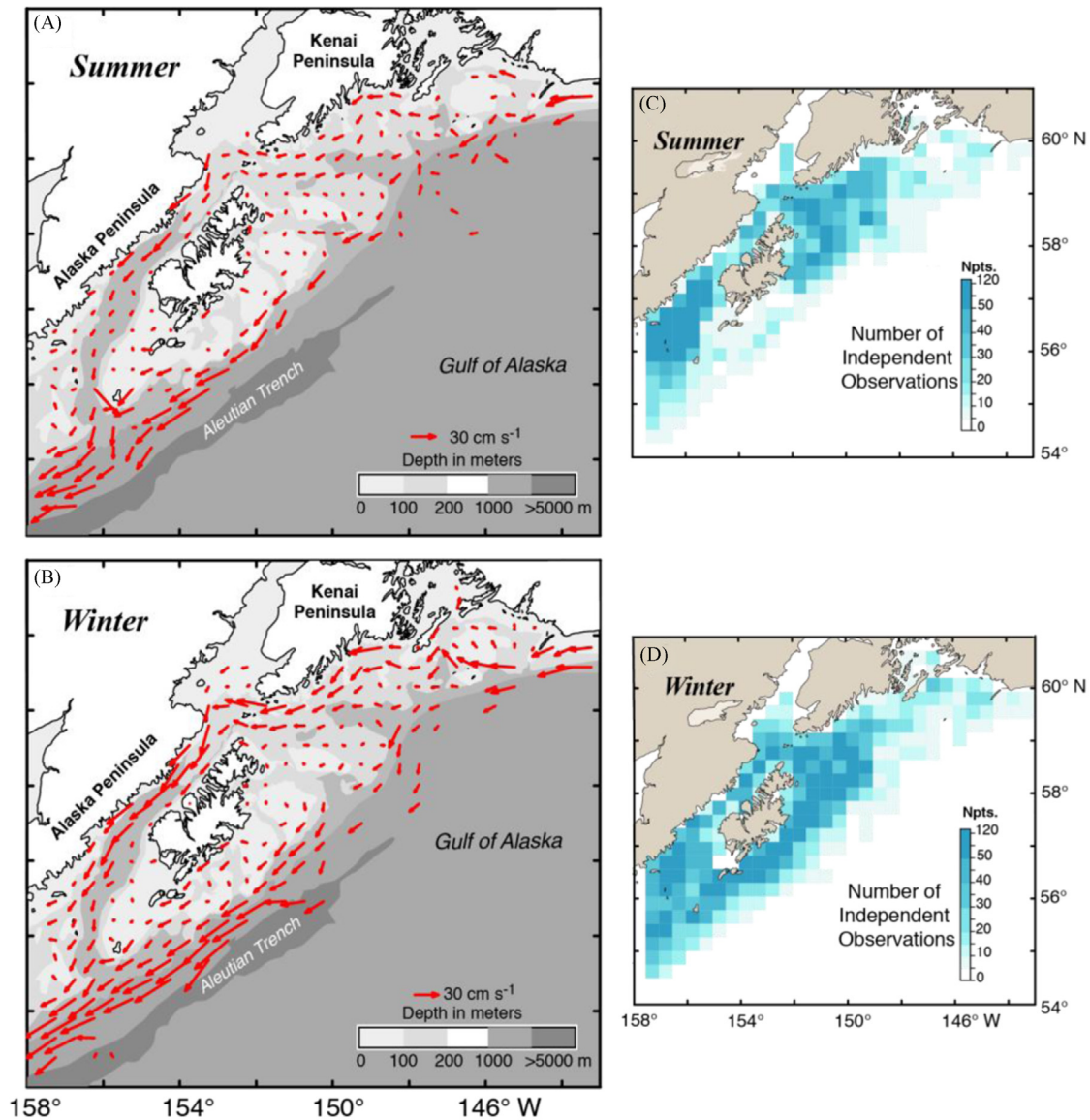
Fig. 4. Maps of currents at ~40 m derived from drifter trajectories for (A) summer and (B) winter. The number of independent estimates for each vector is shown in (C) summer and (D) winter.
