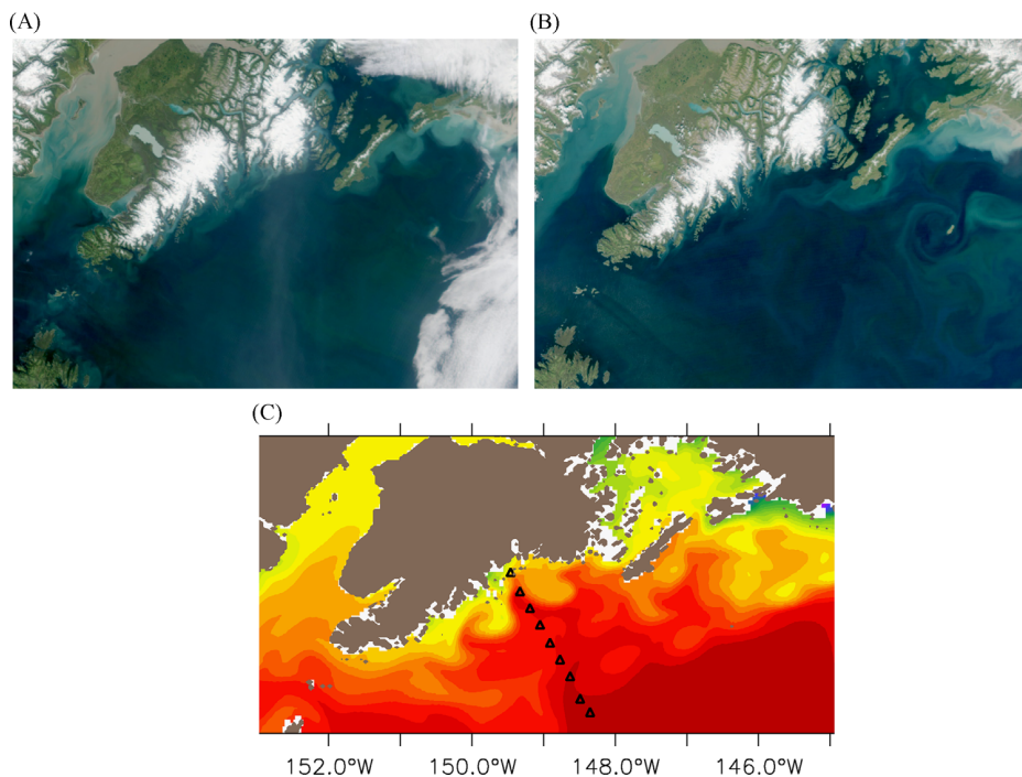
Fig. 10. True color satellite images for (A) August 22, 2001 and (B) September 3, 2002. (C) Modeled 5-m salinity on September 10, 2001. Triangles mark stations on the Seward line.
