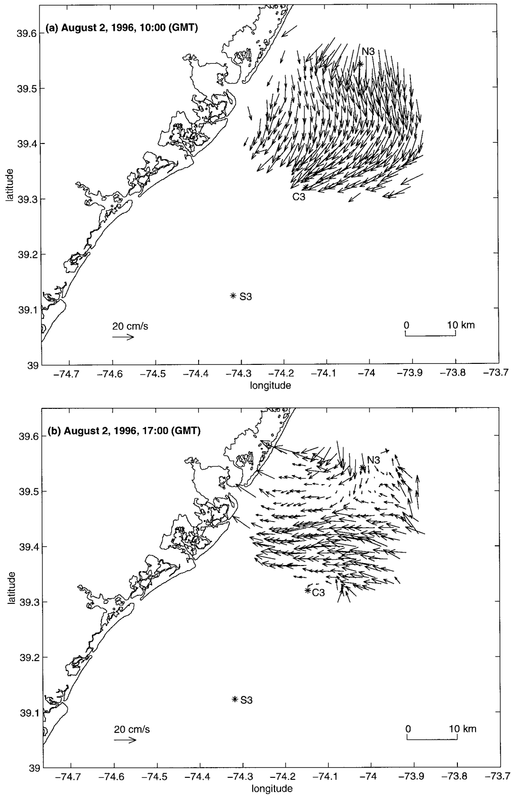
FIG. 7. Detided OSC surface currents measured at (a) 1000 and (b) 1700 UTC 2 Aug 1996.
